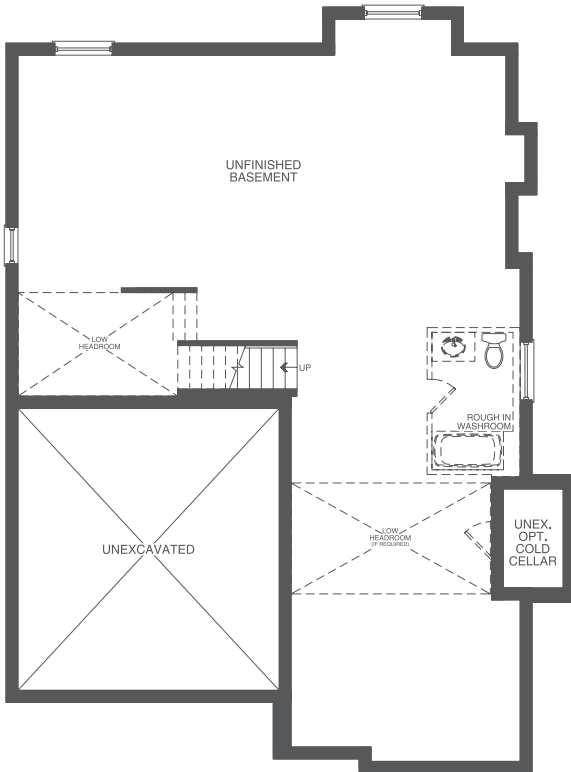
UNFINISHED BASEMENT ELEVATION C 3034 sf
